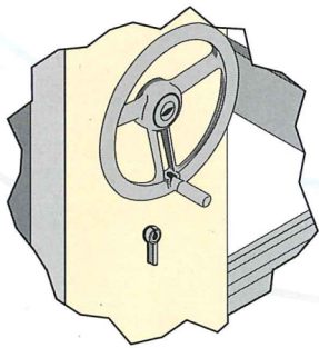
DETAIL D Steering Wheel c/w pull-out handle & safety lock
