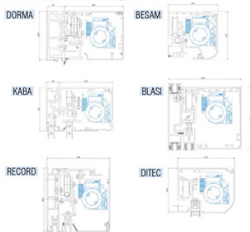
Examples of TINA2 Renovation Kit integration
